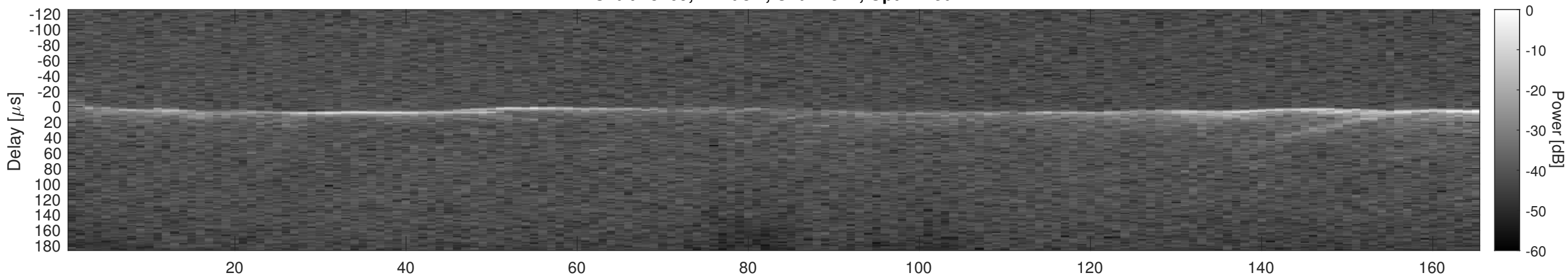
Orbit 18269, Cluttergram
