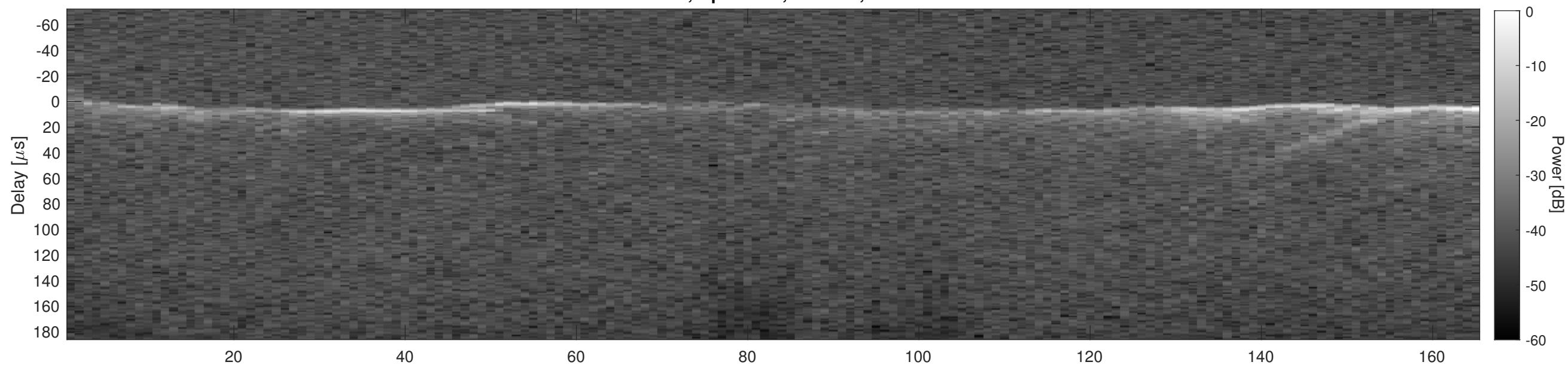
Orbit 18269, Cluttergram
