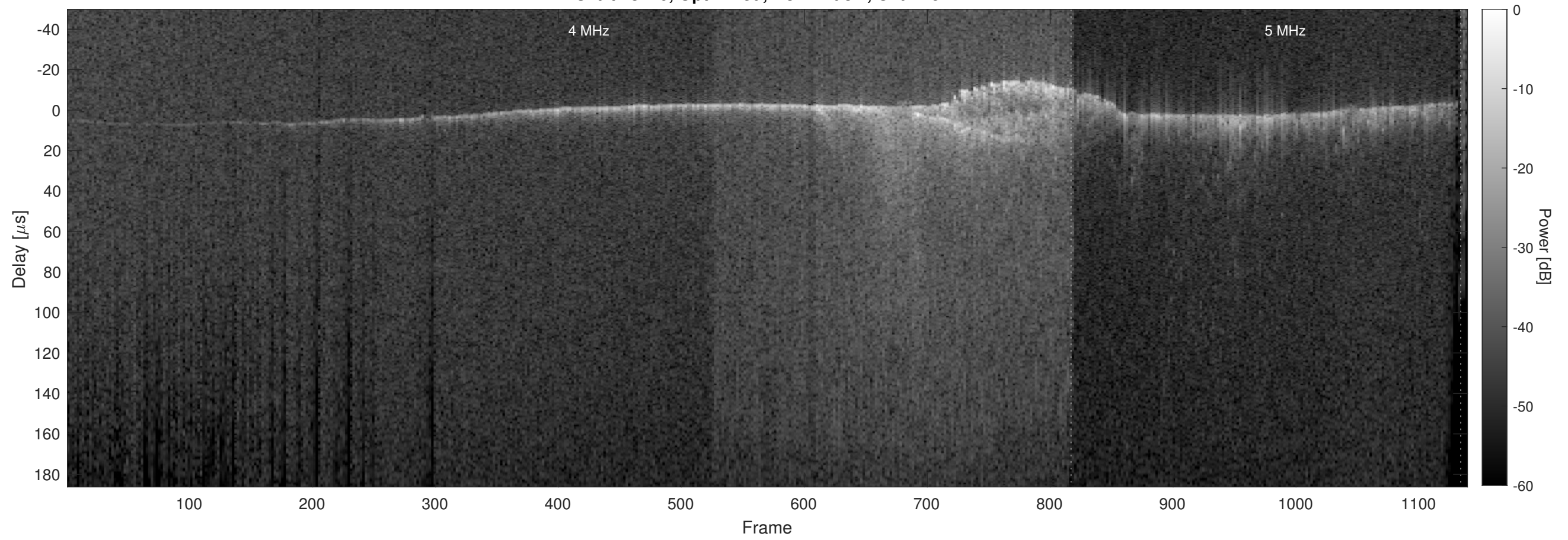
Orbit 18270, Optimized, No Window, Channel 2
