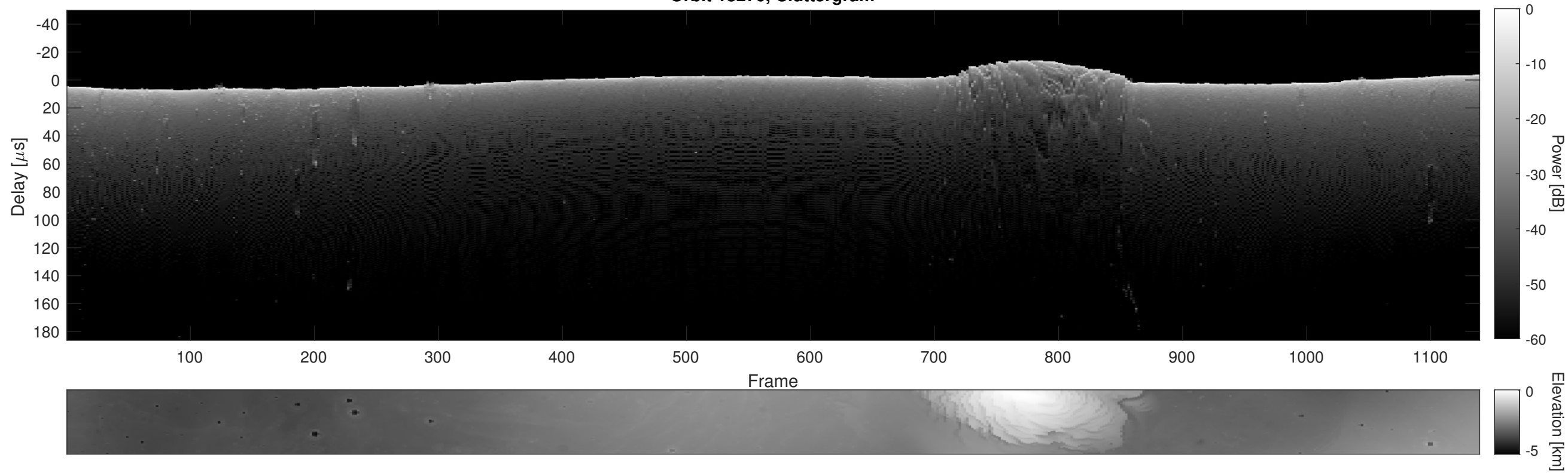
Orbit 18270, Cluttergram
