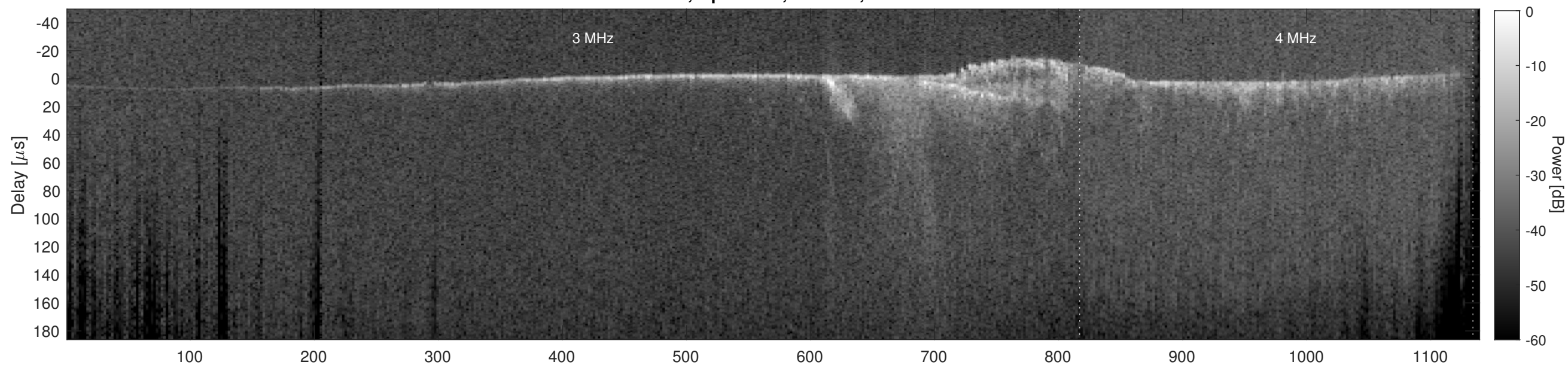
Orbit 18270, Cluttergram
