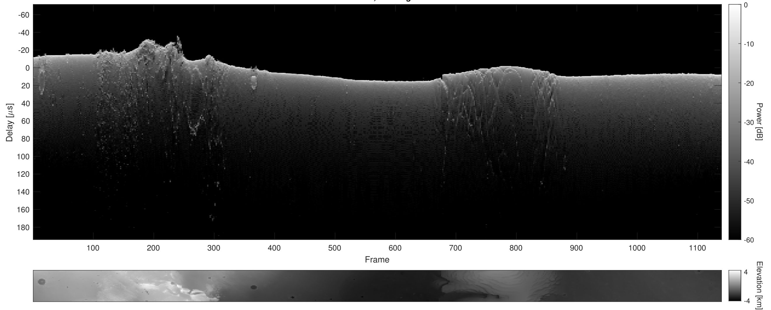
Orbit 18272, Cluttergram
