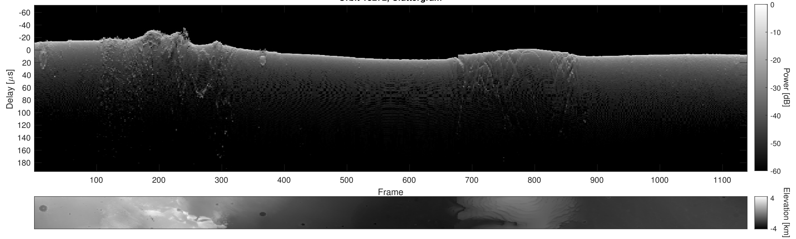
Orbit 18272, Cluttergram
