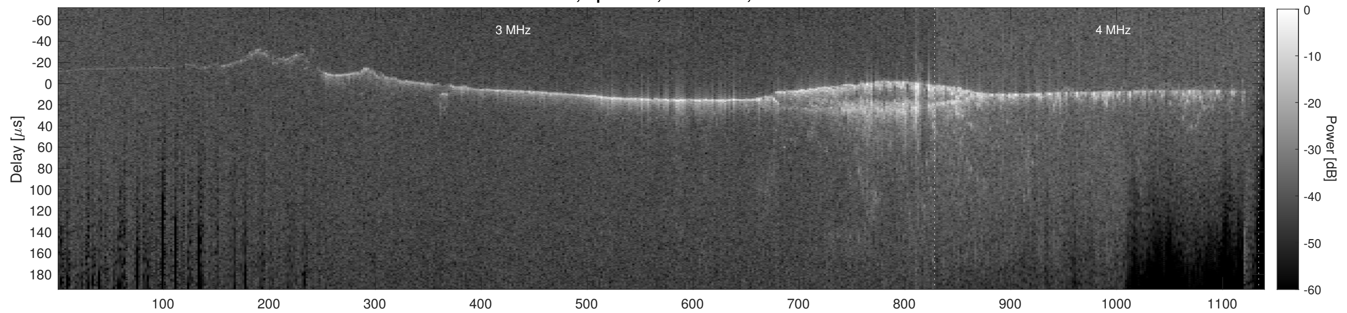
Orbit 18272, Cluttergram
