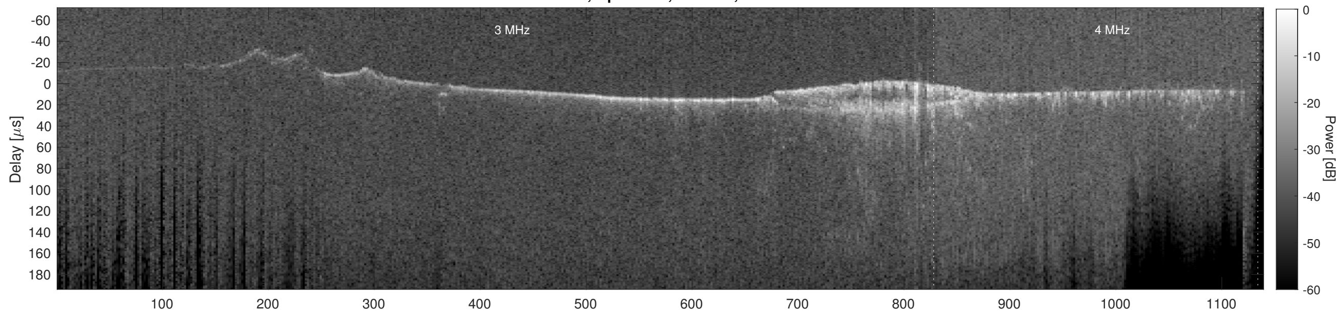
Orbit 18272, Cluttergram
