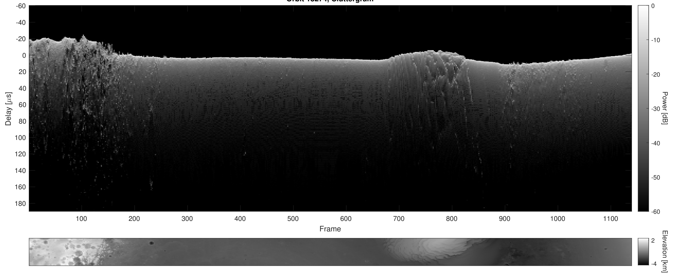
Orbit 18274, Cluttergram
