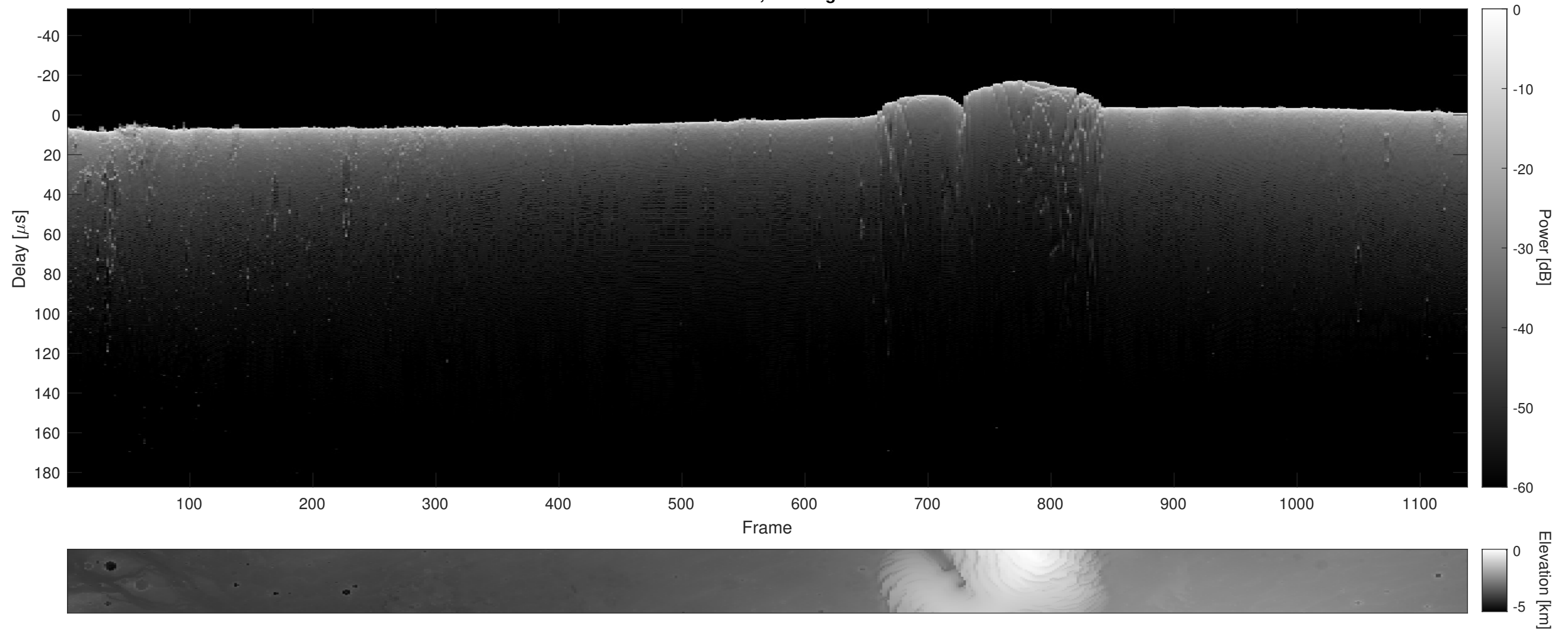
Orbit 18275, Cluttergram
