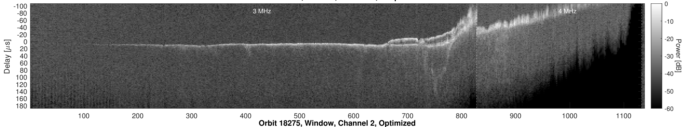
Orbit 18275, Window, Channel 2, Chapman
