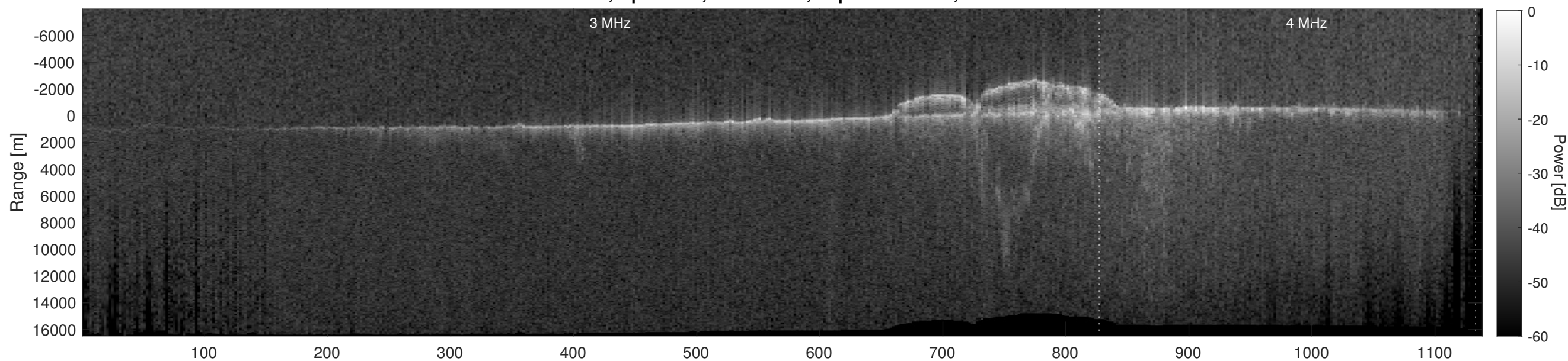
Orbit 18275, Depth-Corrected Cluttergram
