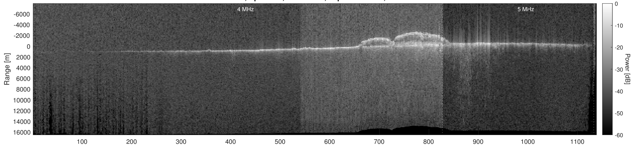
Orbit 18275, Optimized, No Window, Depth-Corrected, Channel 2
