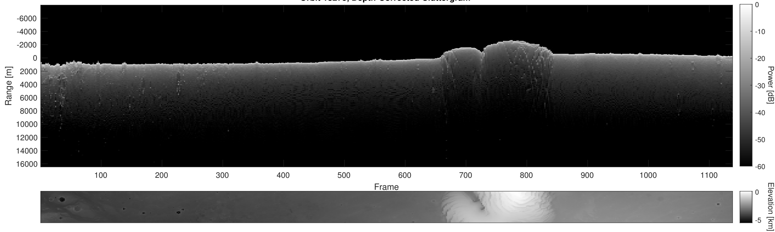
Orbit 18275, Depth-Corrected Cluttergram
