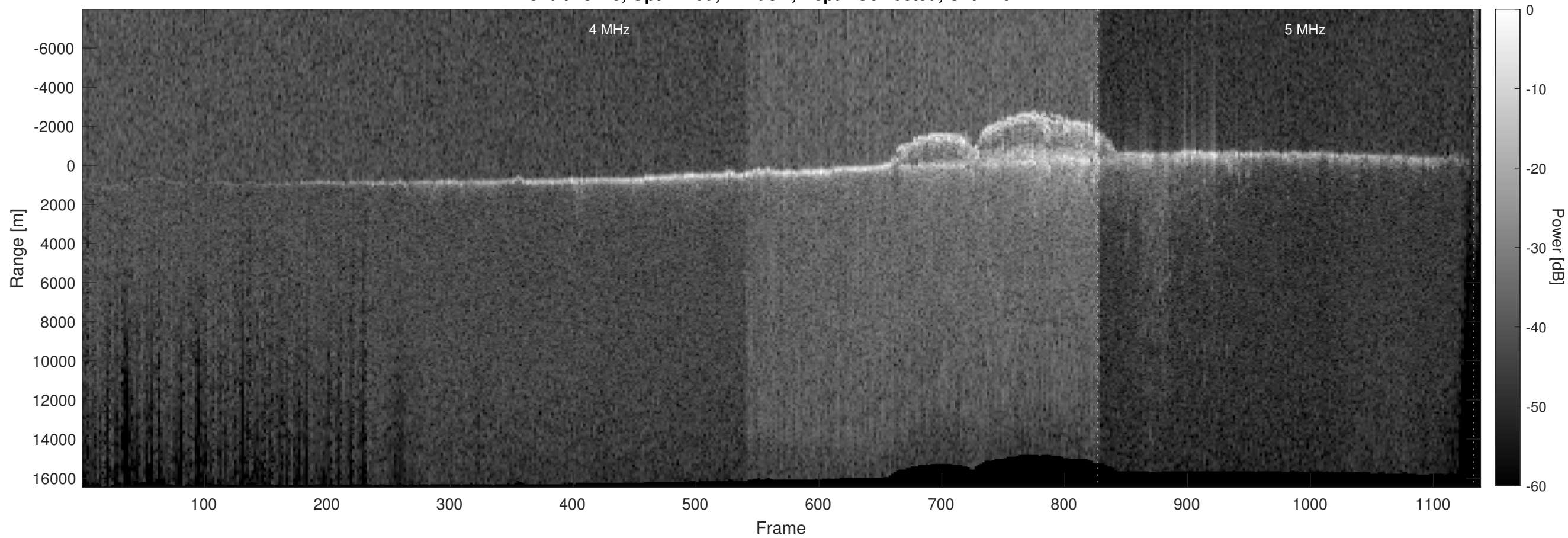
Orbit 18275, Optimized, Window, Depth-Corrected, Channel 2
