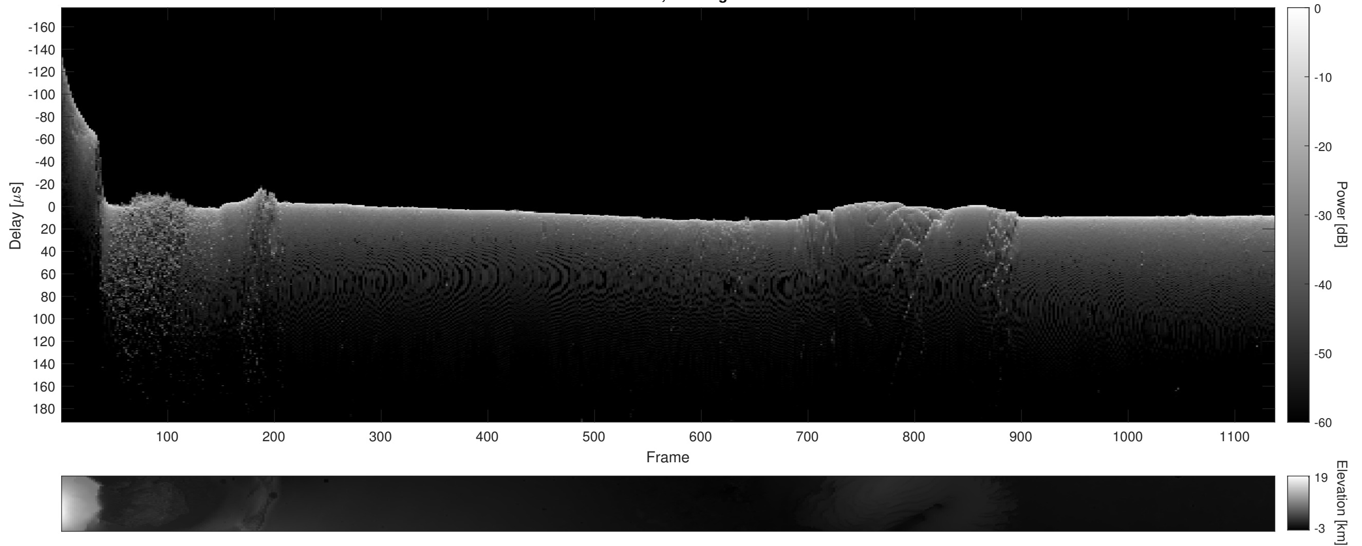
Orbit 18276, Cluttergram
