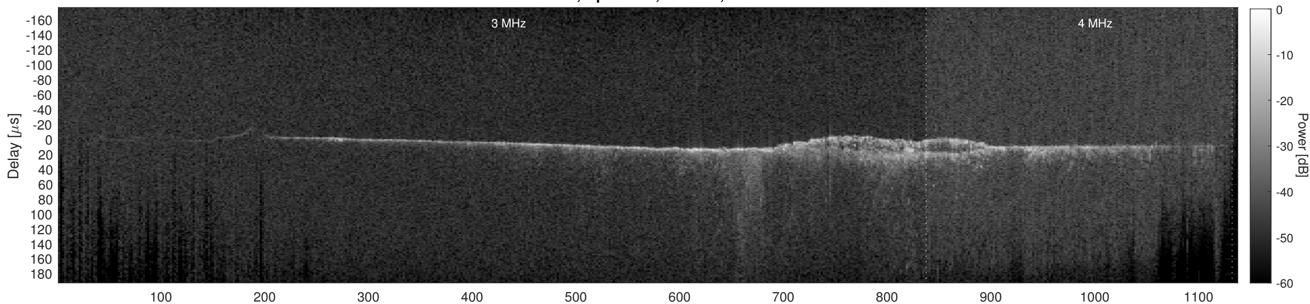
Orbit 18276, Cluttergram
