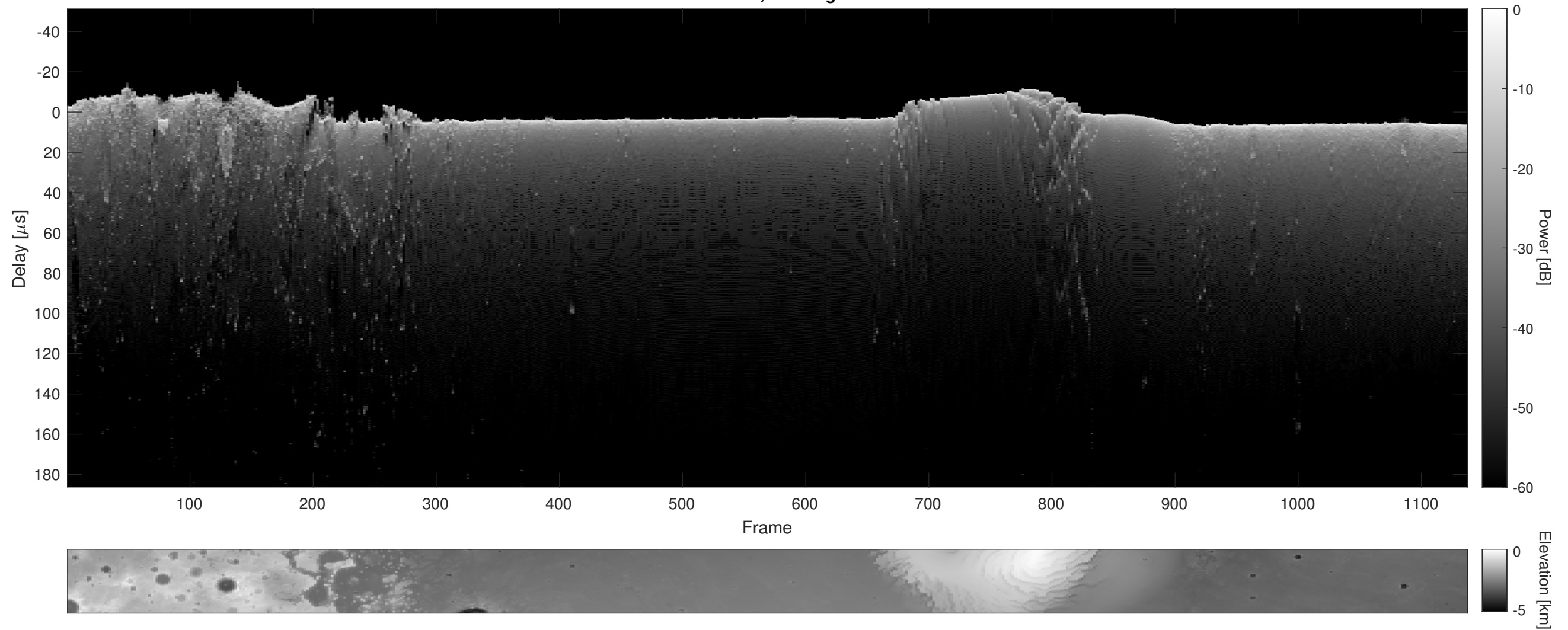
Orbit 18278, Cluttergram
