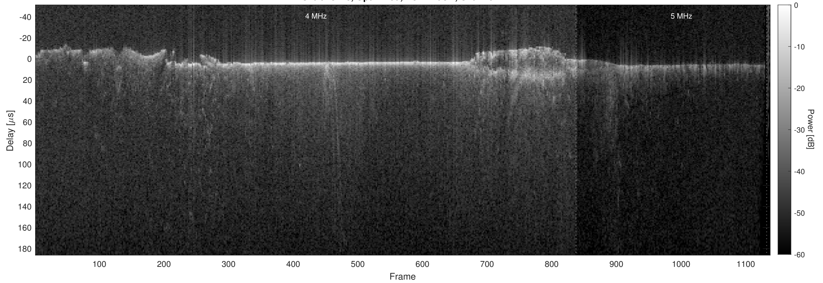
Orbit 18278, Optimized, No Window, Channel 2
