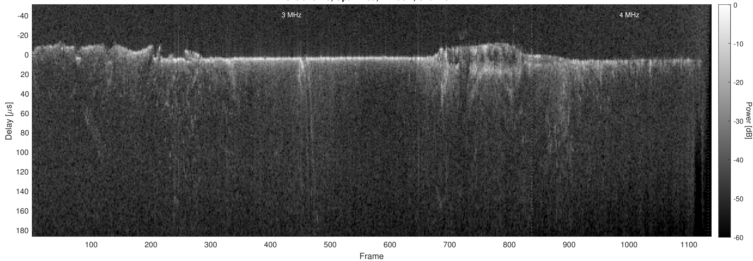
Orbit 18278, Optimized, Window, Channel 2
