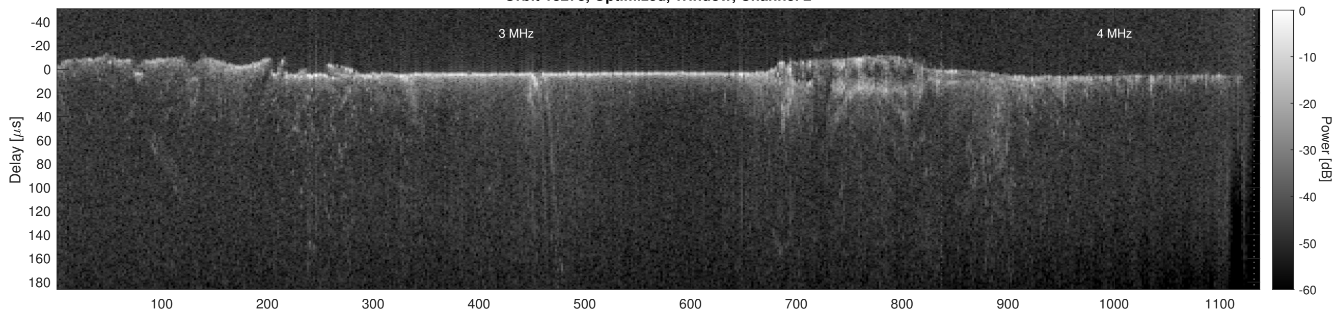
Orbit 18278, Cluttergram
