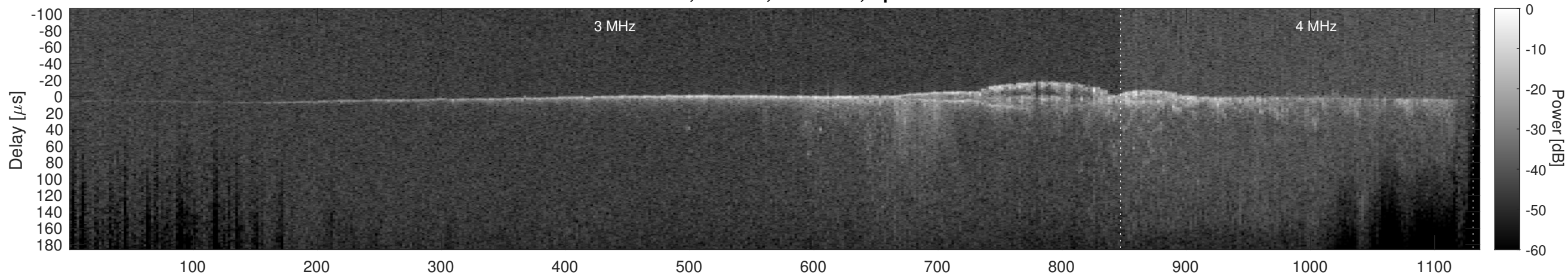
Orbit 18280, Cluttergram
