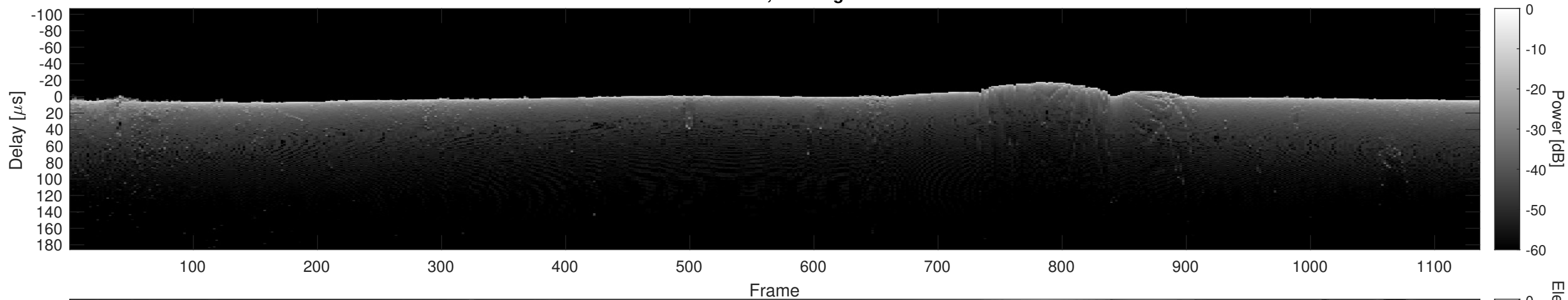
Orbit 18280, Cluttergram
