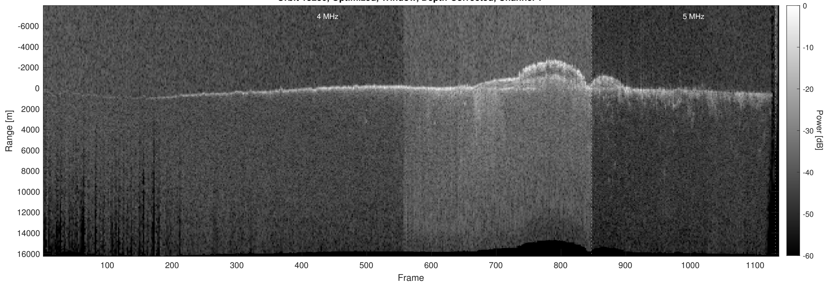
Orbit 18280, Optimized, Window, Depth-Corrected, Channel 2
