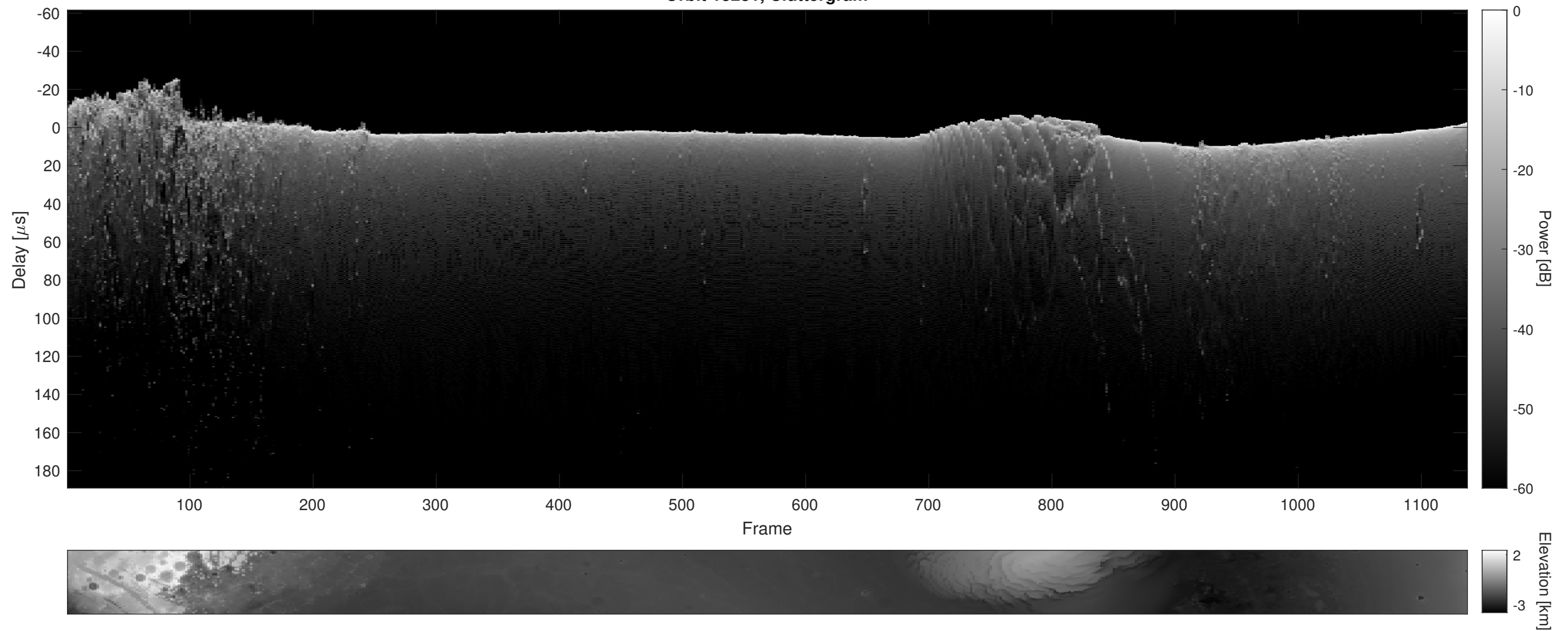
Orbit 18281, Cluttergram
