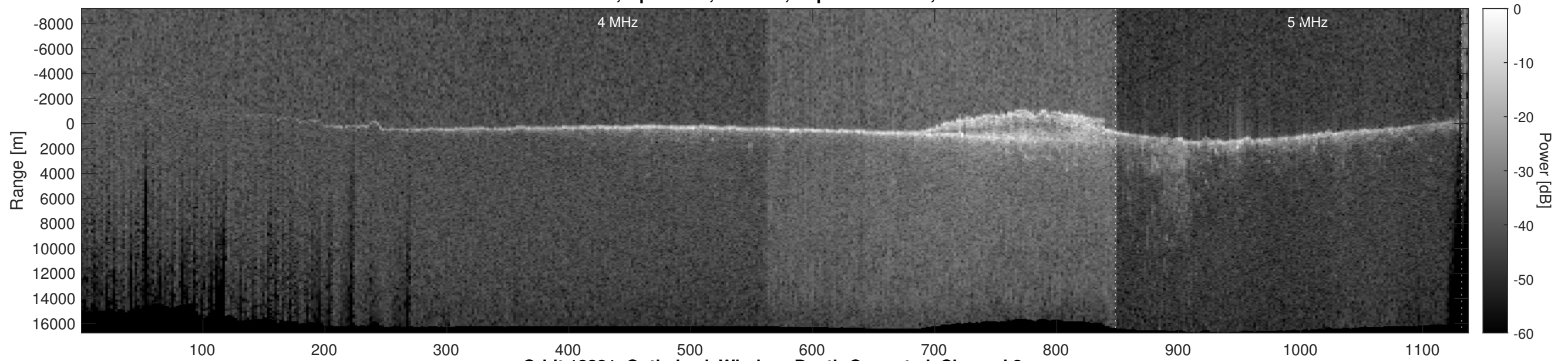
Orbit 18281, Optimized, Window, Depth-Corrected, Channel 2
