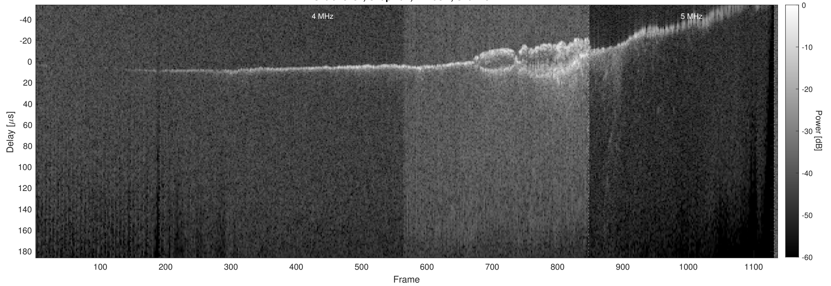
Orbit 18282, Chapman, Window, Channel 2
