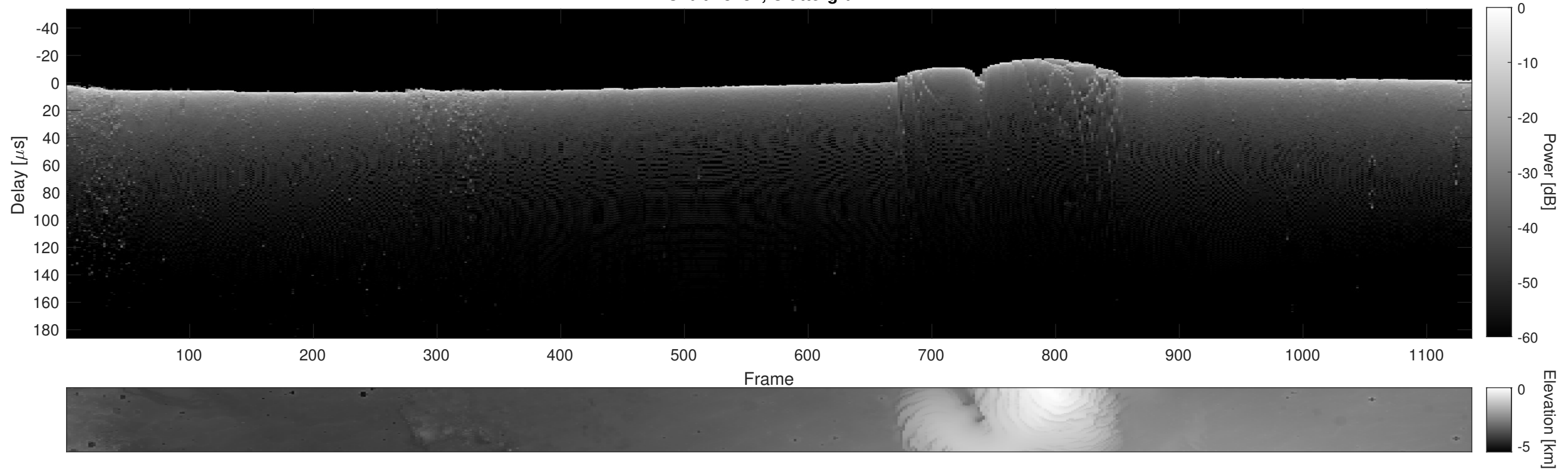
Orbit 18282, Cluttergram
