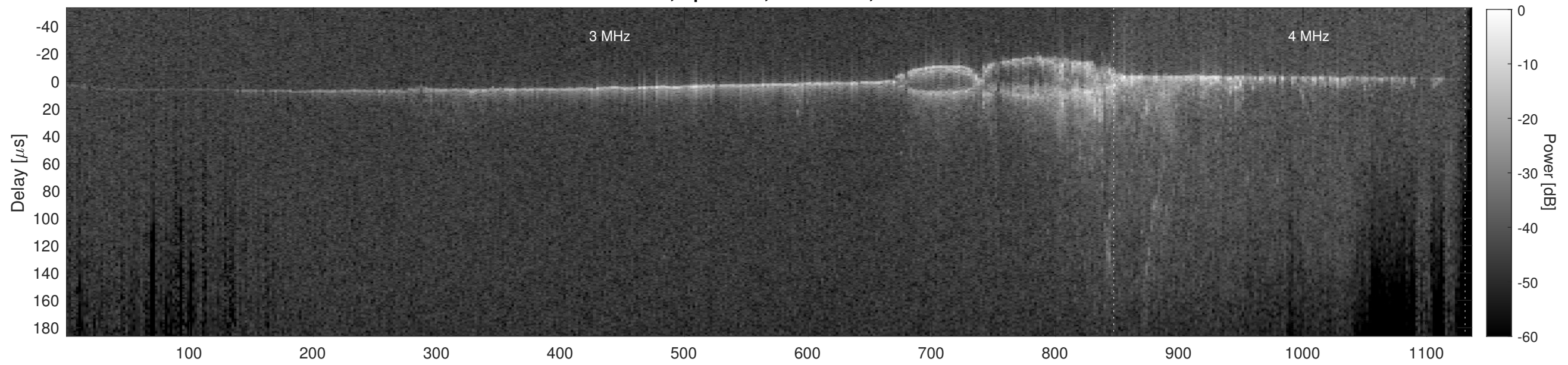
Orbit 18282, Cluttergram
