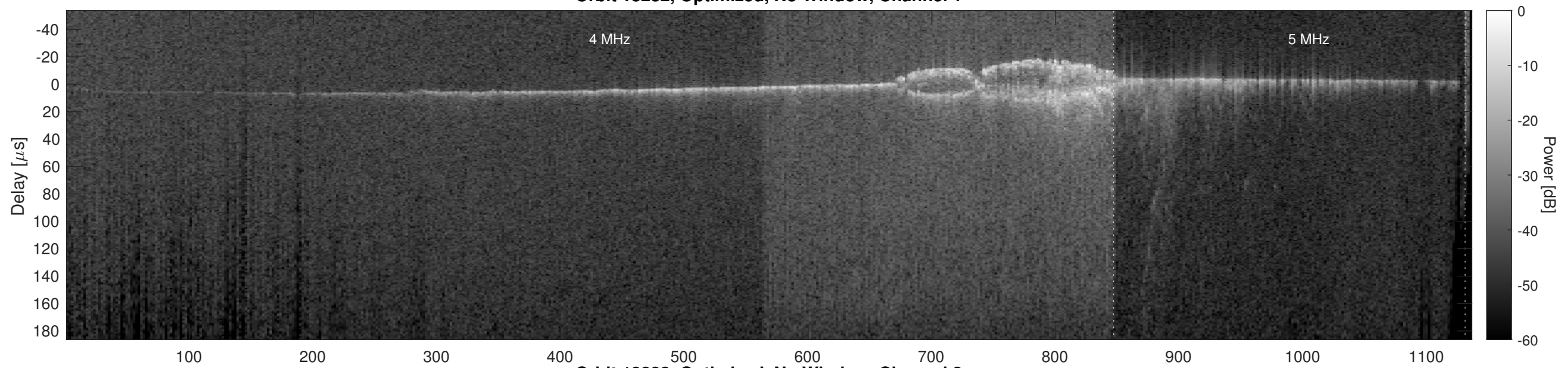
Orbit 18282, Optimized, No Window, Channel 2
