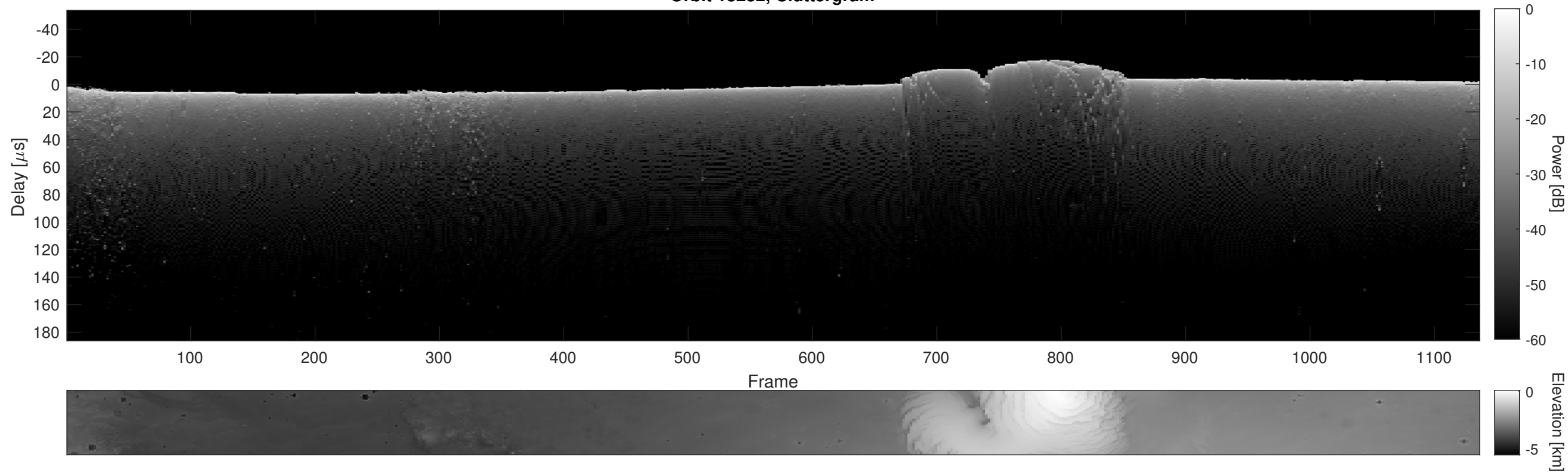
Orbit 18282, Cluttergram
