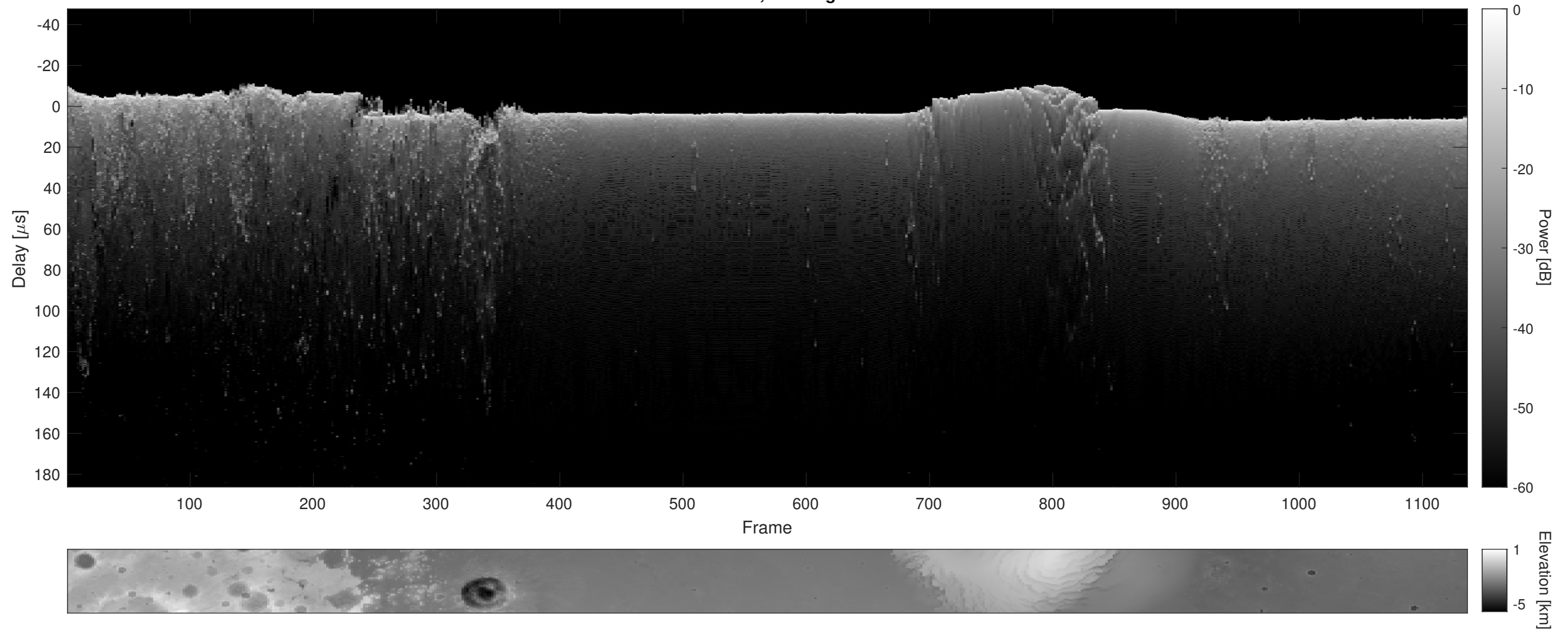
Orbit 18285, Cluttergram
