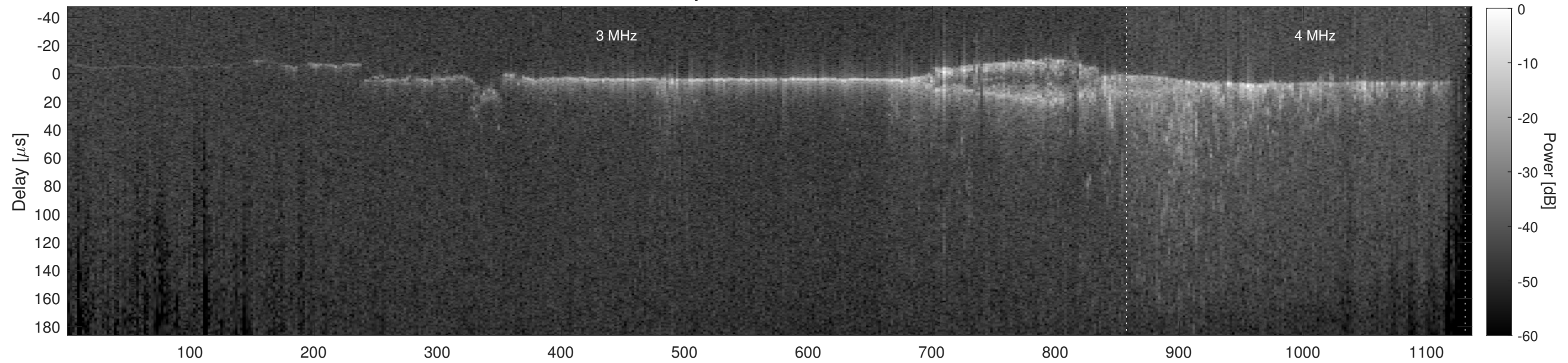
Orbit 18285, Cluttergram
