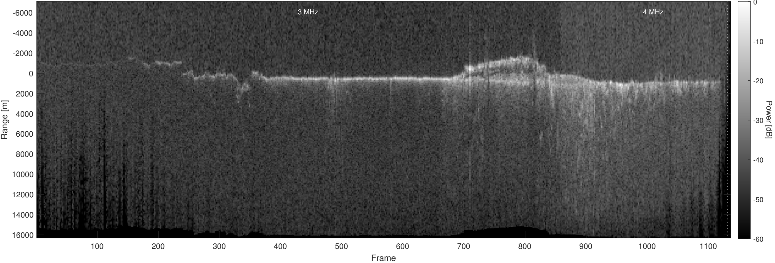
Orbit 18285, Optimized, Window, Depth-Corrected, Channel 2
