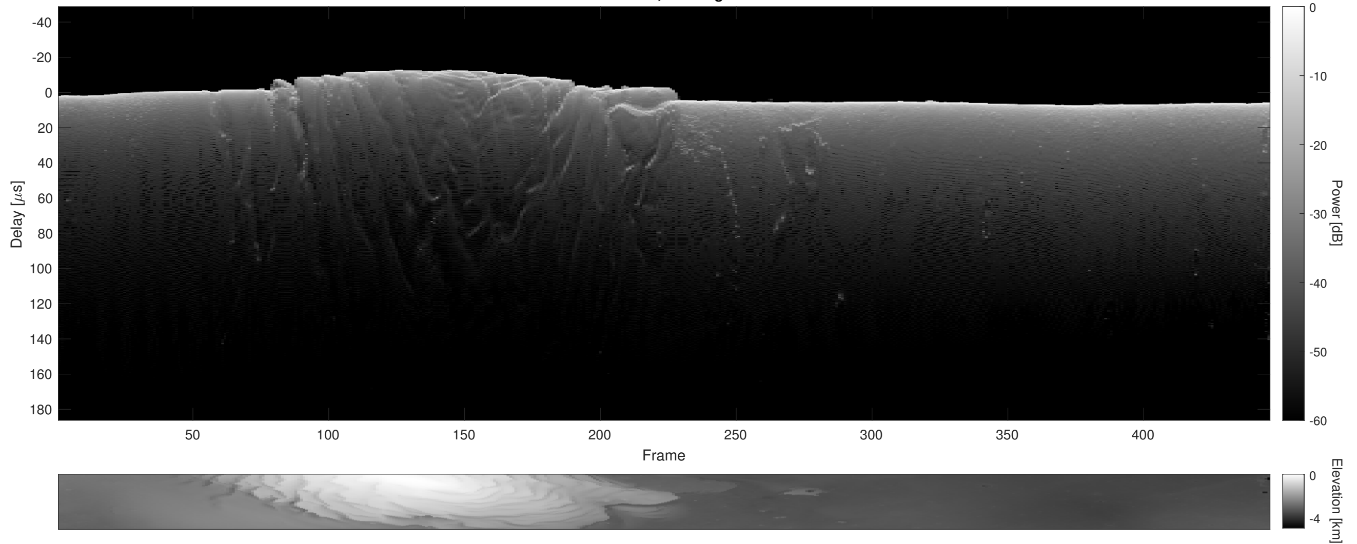
Orbit 18298, Cluttergram
