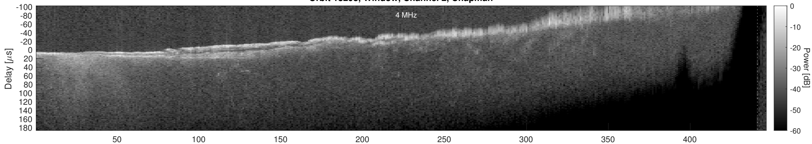
Orbit 18298, Window, Channel 2, Optimized
