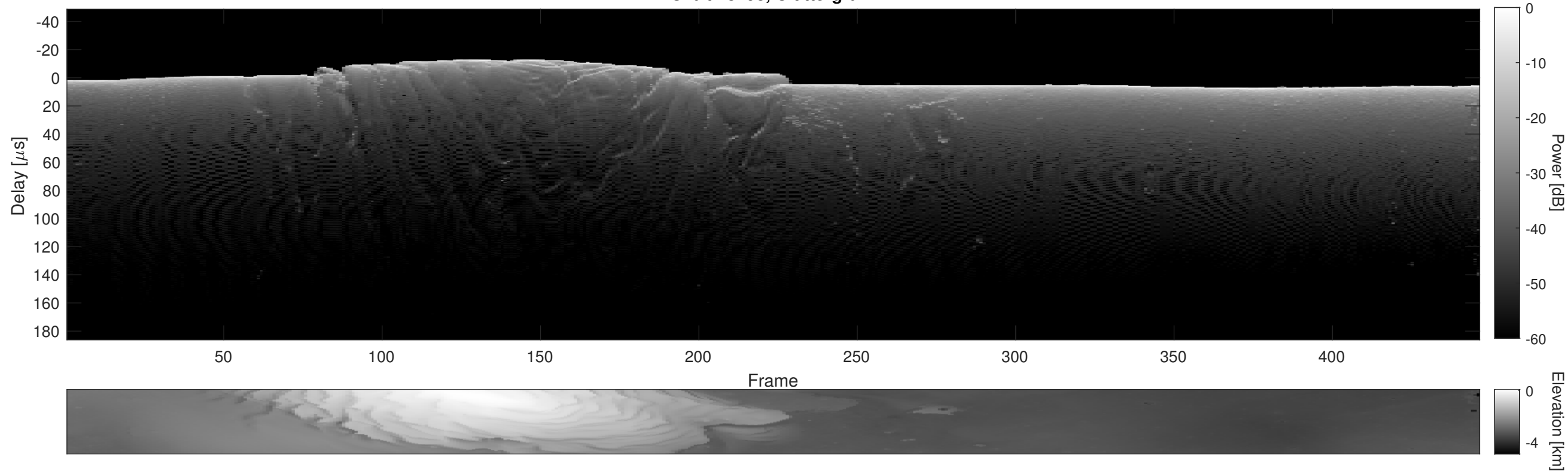
Orbit 18298, Cluttergram
