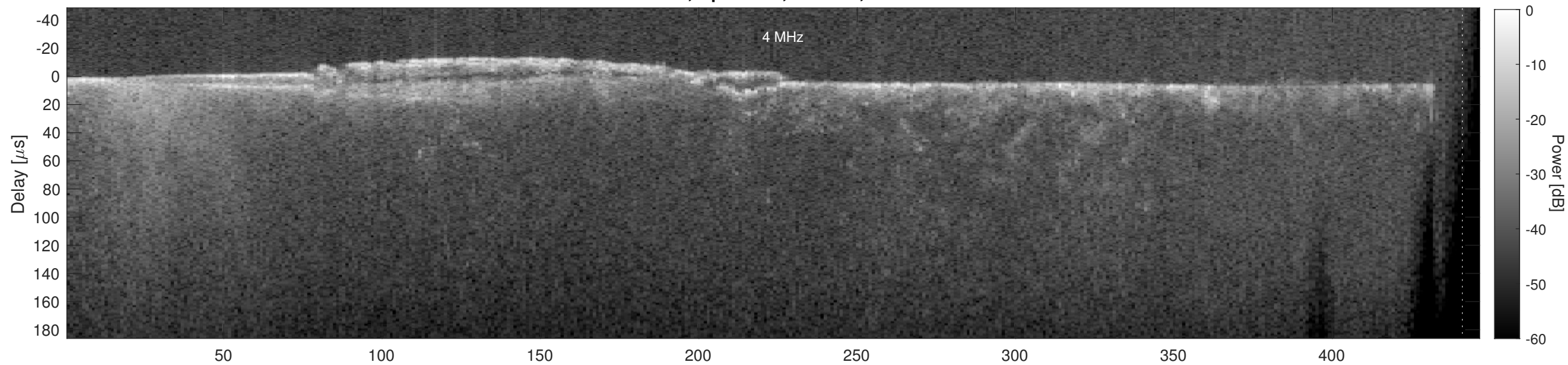
Orbit 18298, Cluttergram
