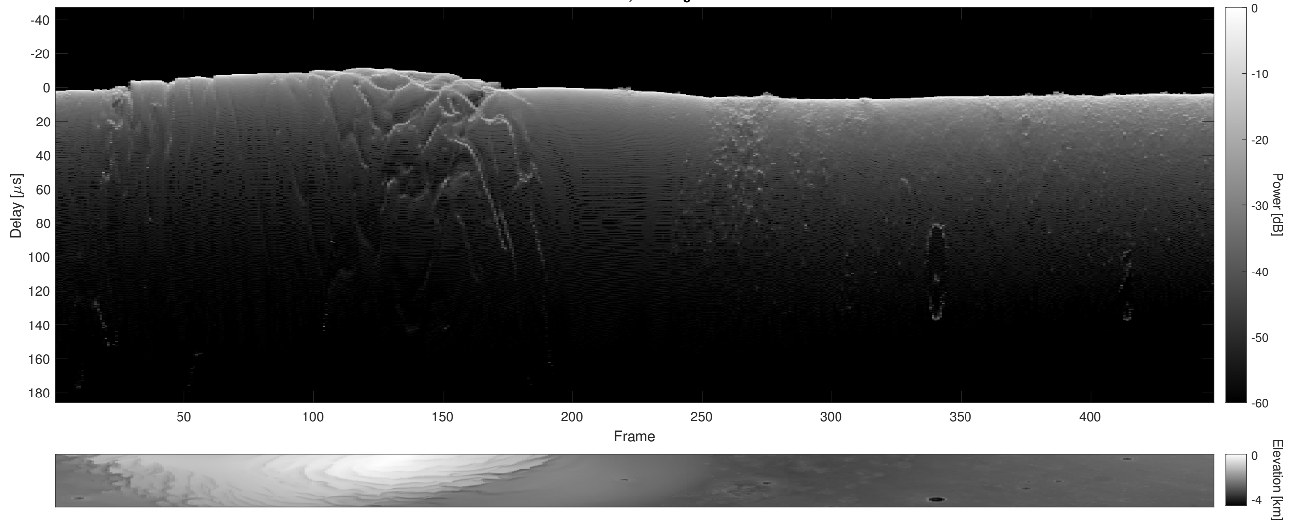
Orbit 18299, Cluttergram
