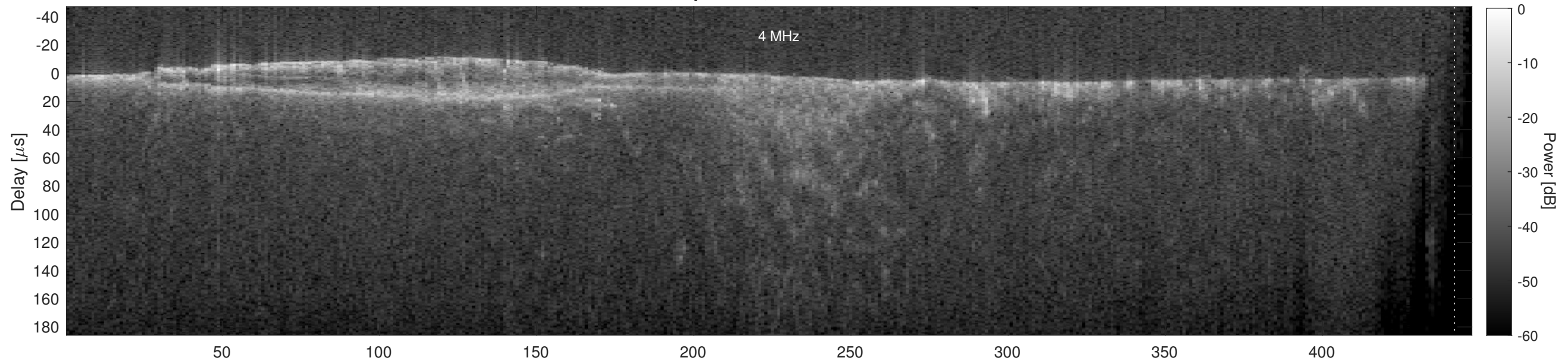
Orbit 18299, Cluttergram
