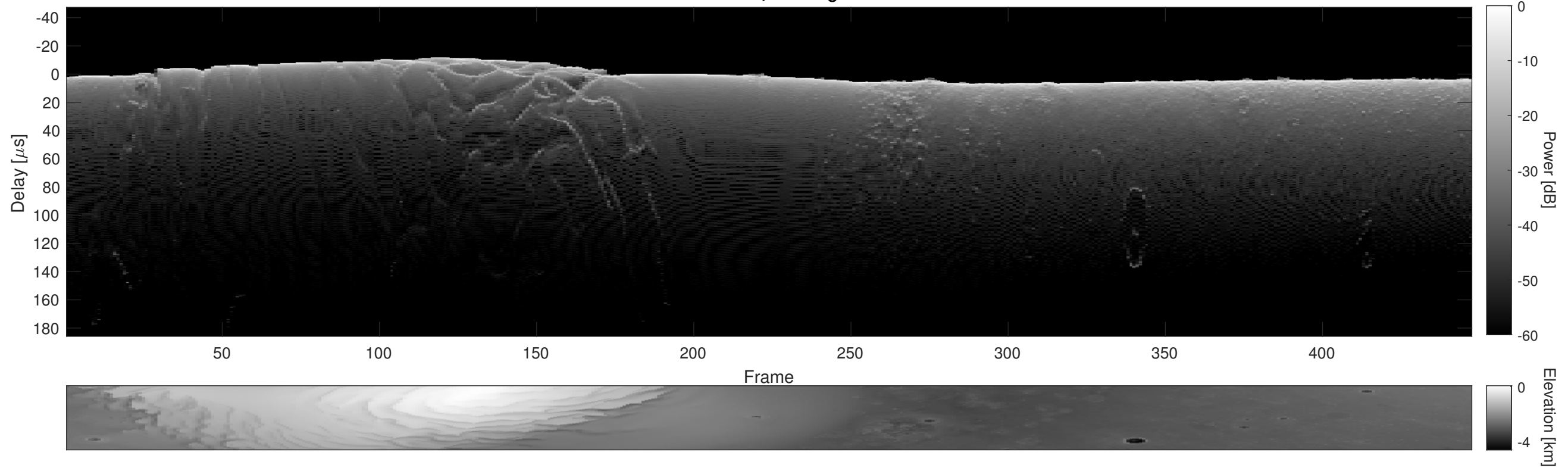
Orbit 18299, Cluttergram
