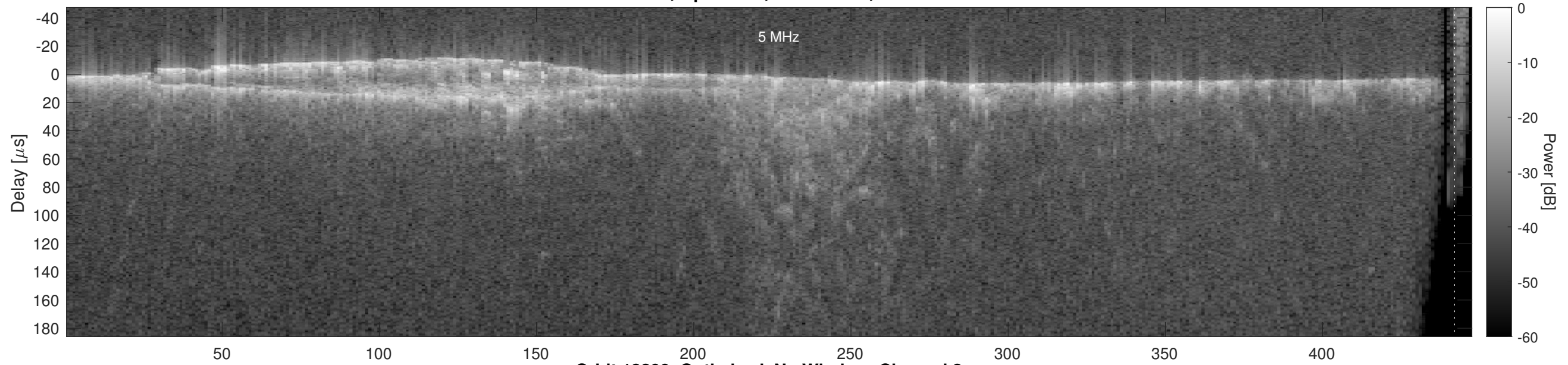
Orbit 18299, Optimized, No Window, Channel 2
