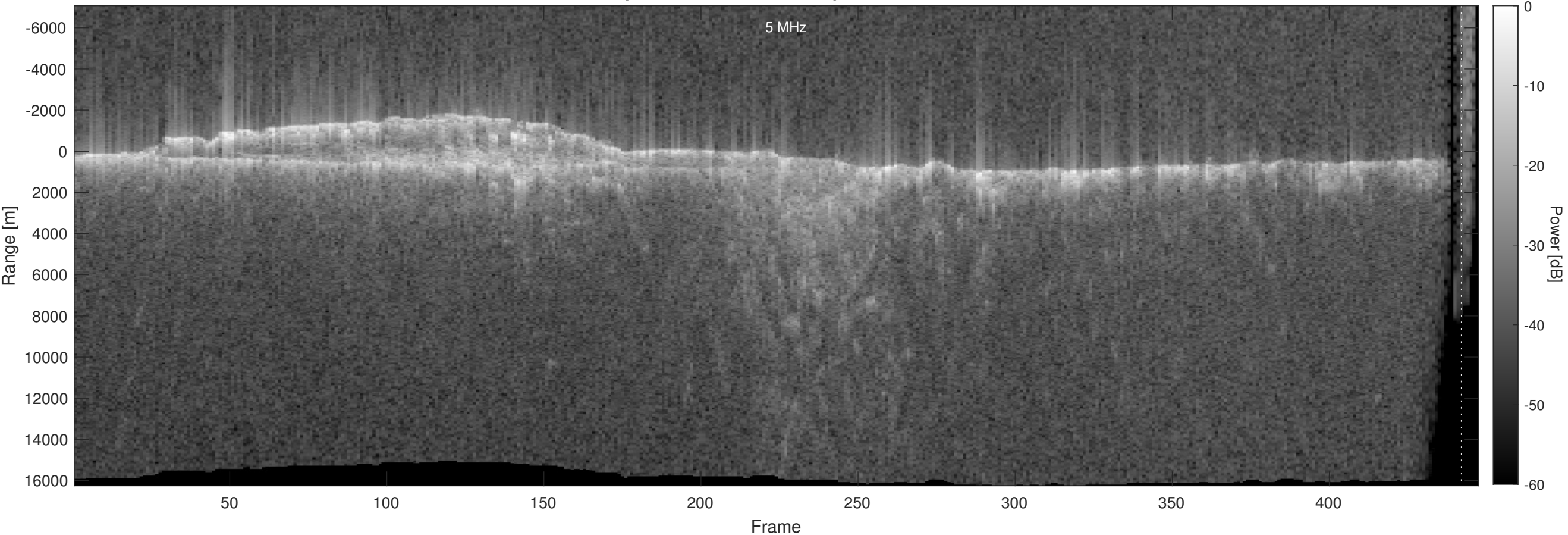
Orbit 18299, Optimized, No Window, Depth-Corrected, Channel 2
