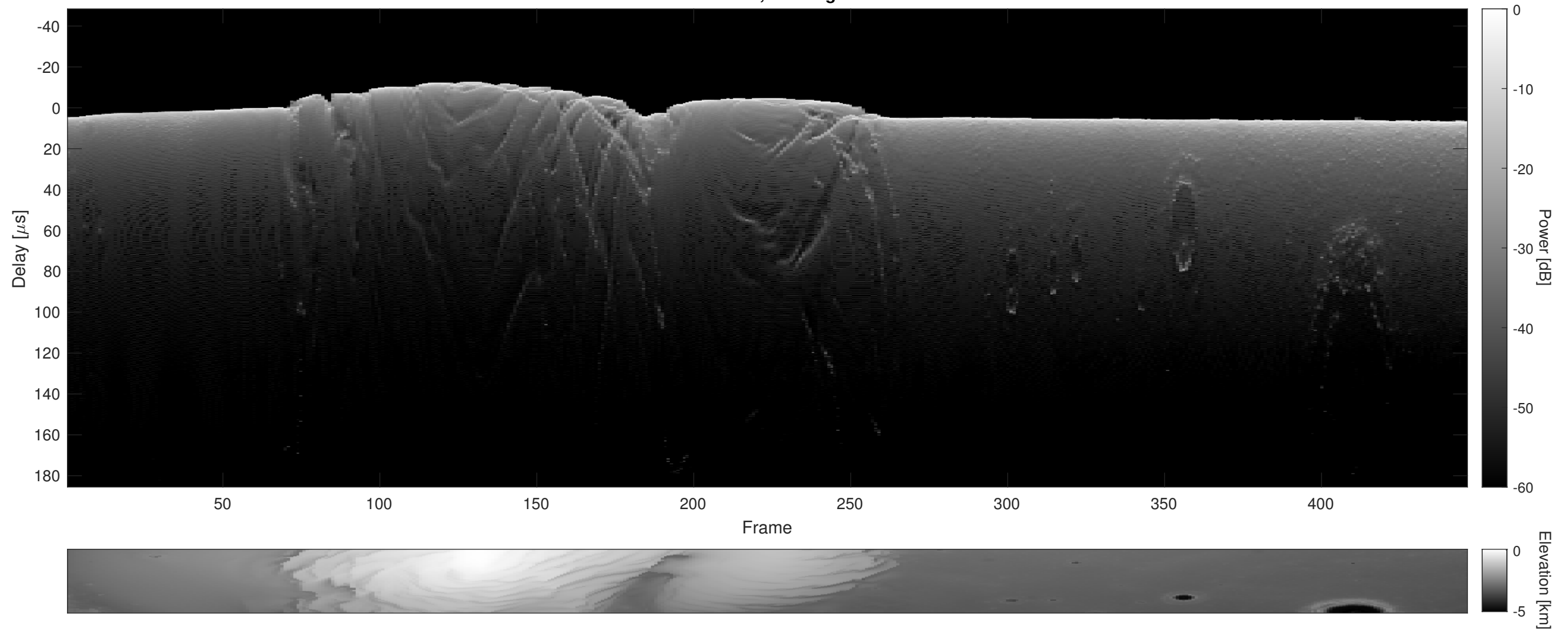
Orbit 18301, Cluttergram
