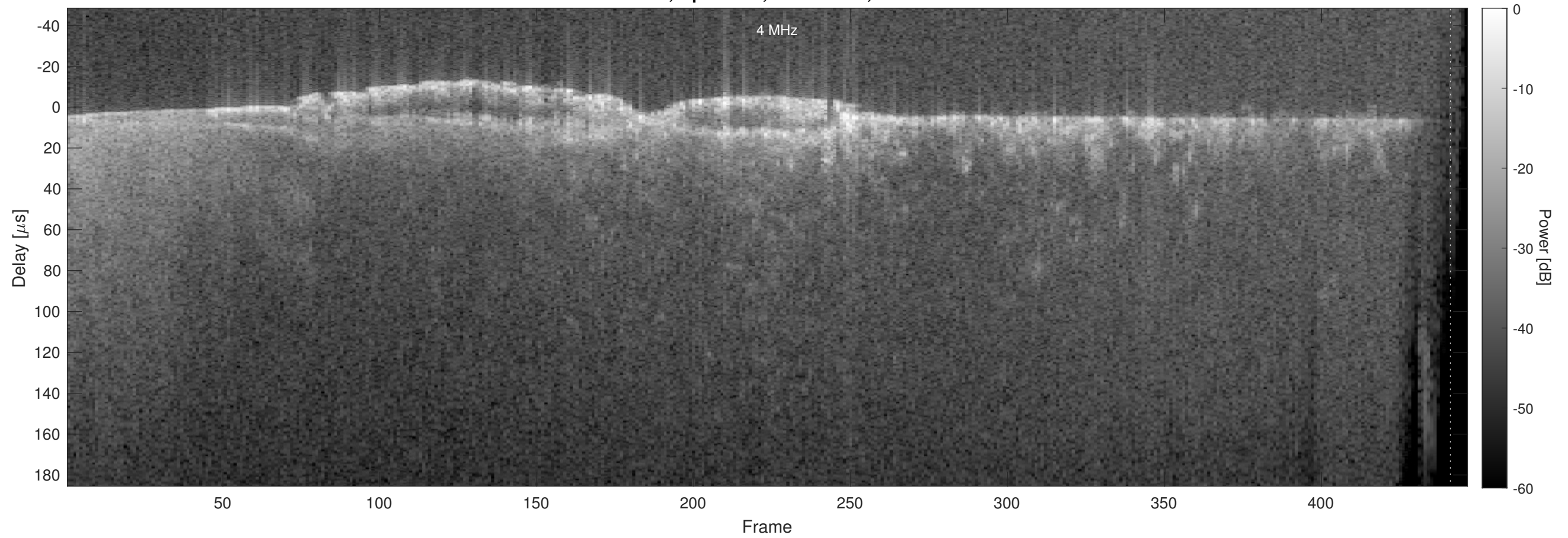
Orbit 18301, Optimized, No Window, Channel 2
