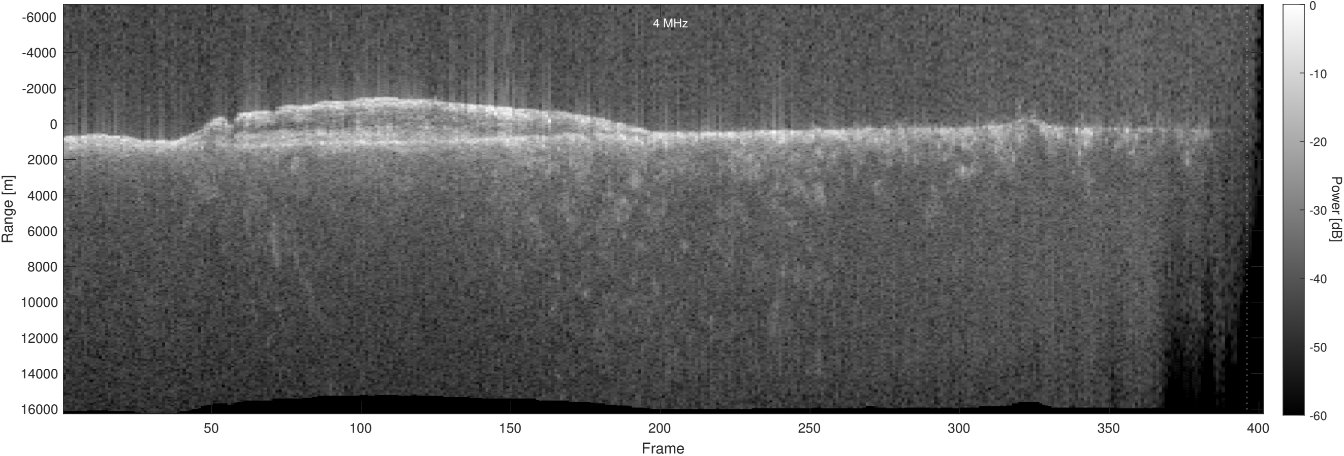
Orbit 18307, Optimized, No Window, Depth-Corrected, Channel 2
