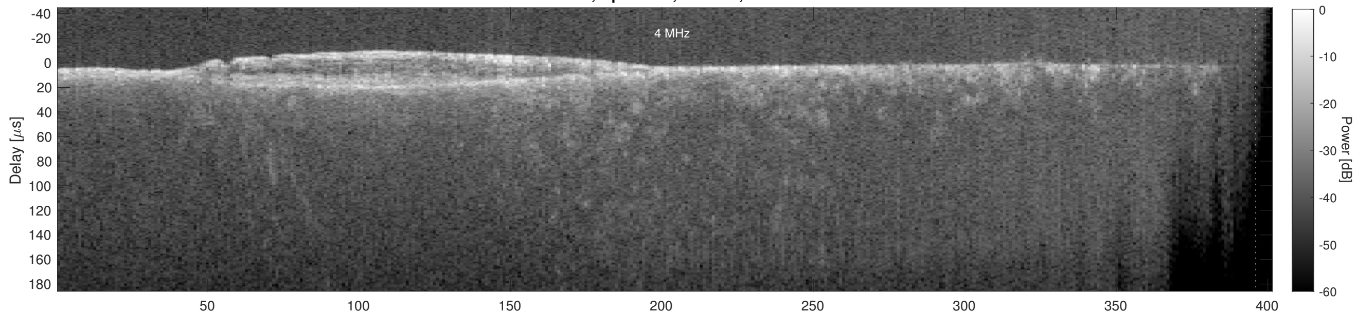
Orbit 18307, Cluttergram
