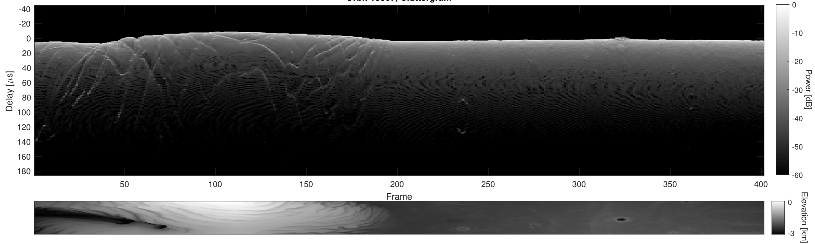
Orbit 18307, Cluttergram
