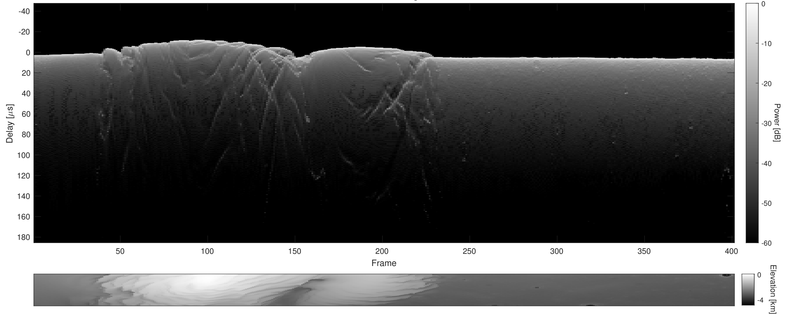
Orbit 18308, Cluttergram
