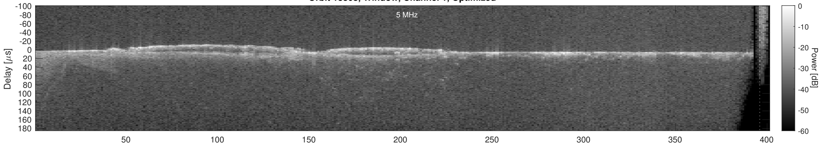
Orbit 18308, Cluttergram
