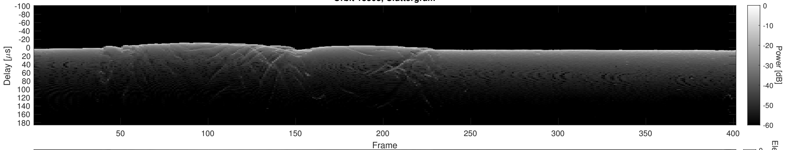
Orbit 18308, Cluttergram
