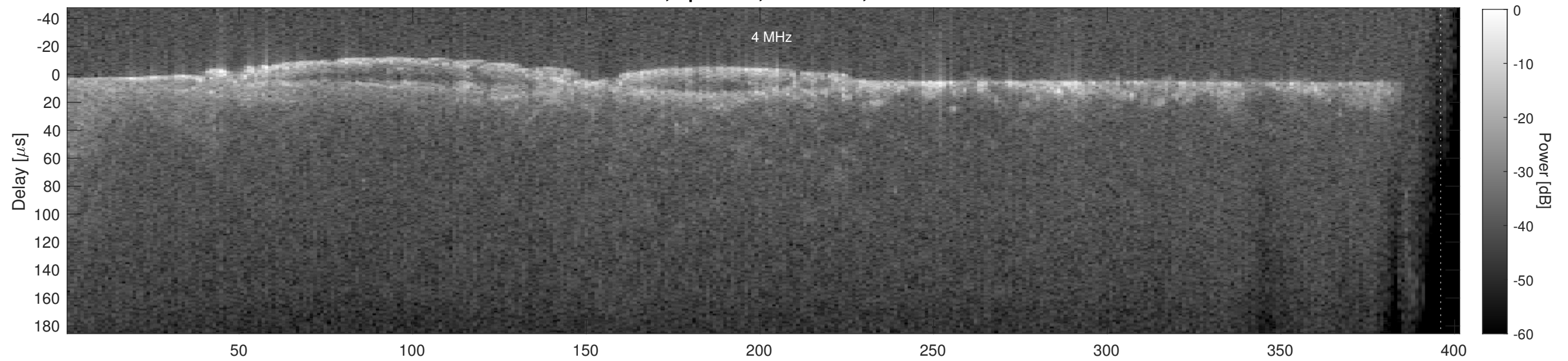
Orbit 18308, Cluttergram
