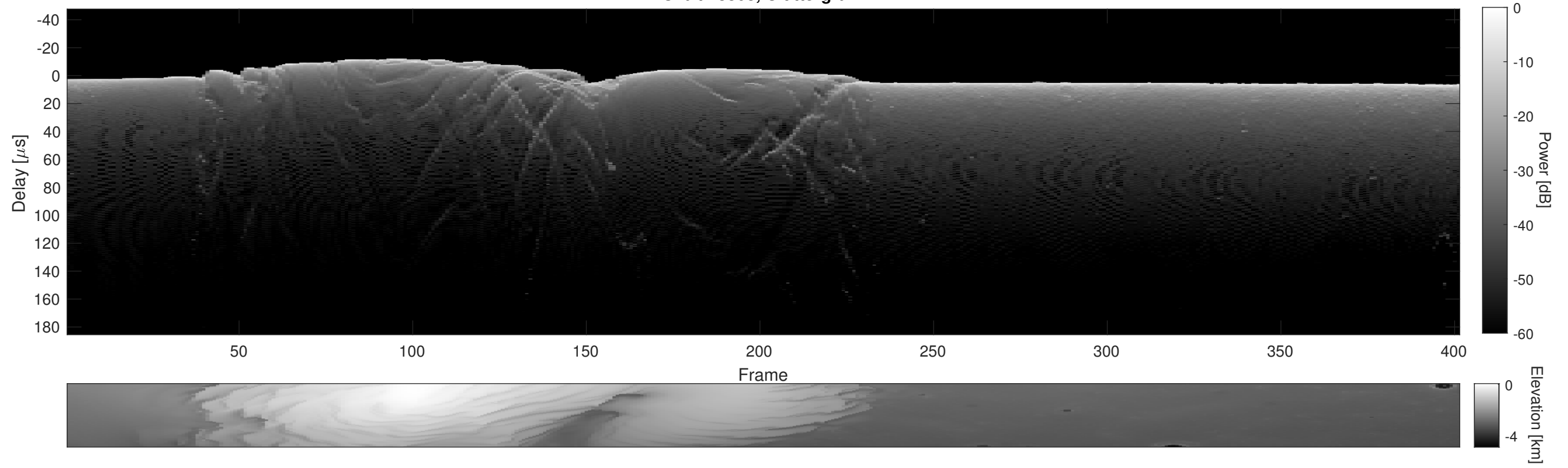
Orbit 18308, Cluttergram
