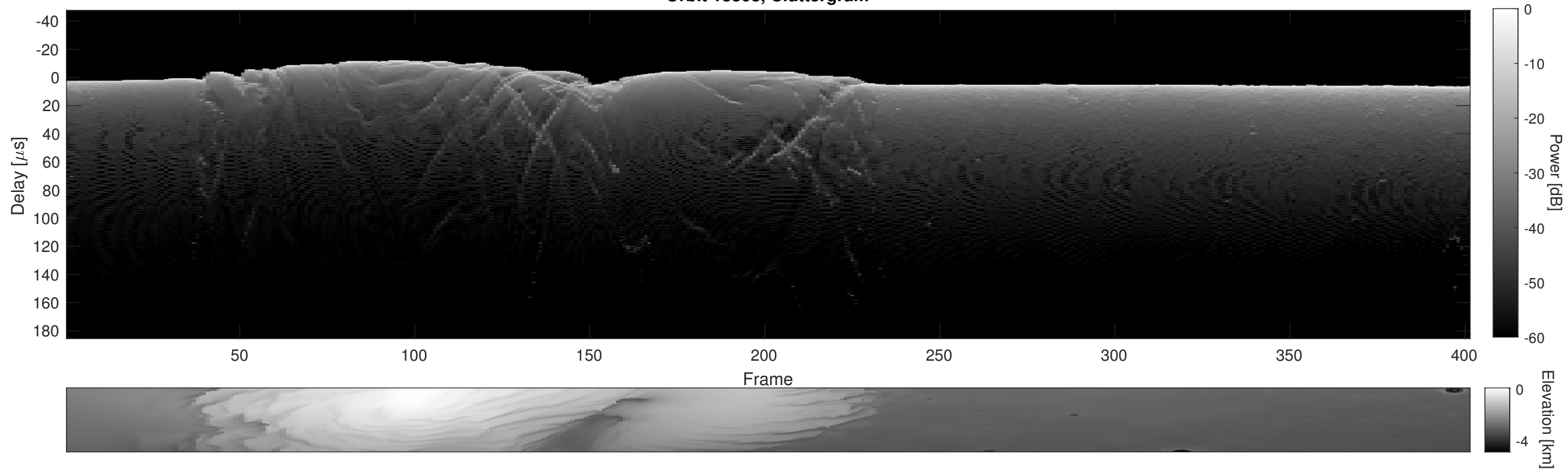
Orbit 18308, Cluttergram
