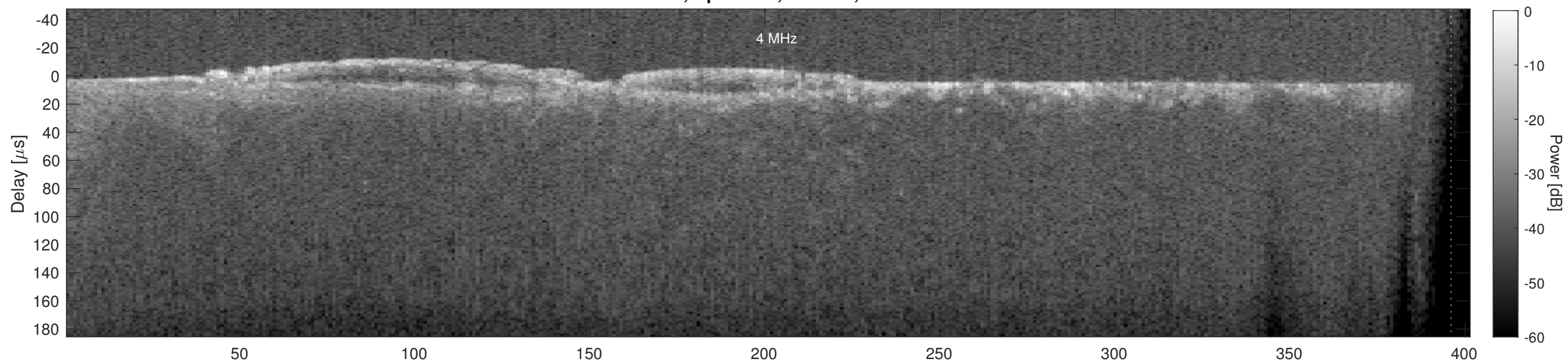
Orbit 18308, Cluttergram
