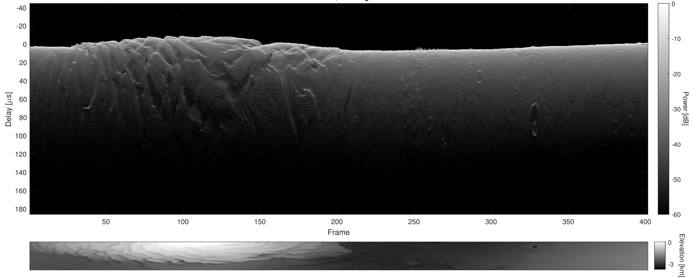
Orbit 18309, Cluttergram
