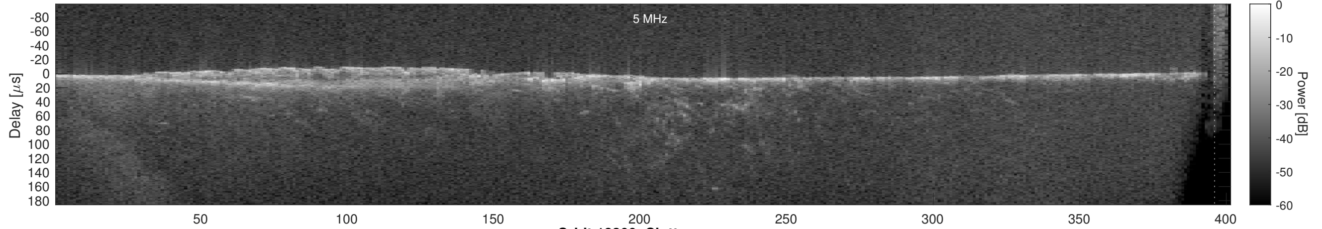
Orbit 18309, Cluttergram
