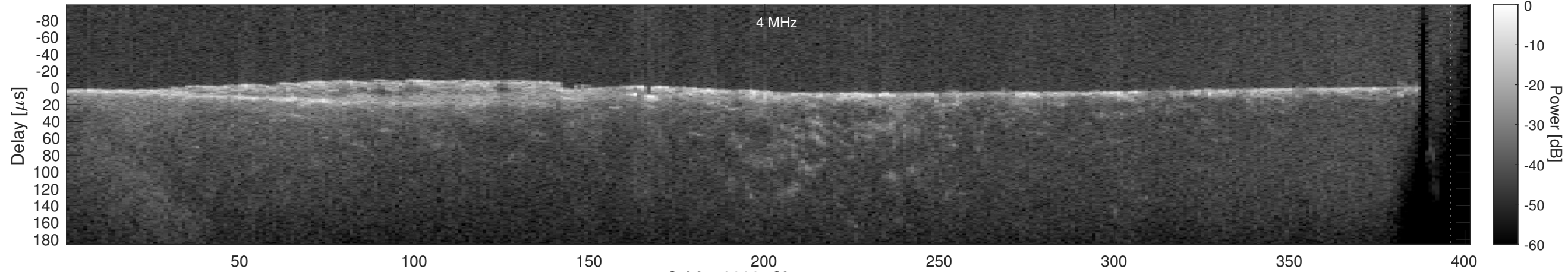
Orbit 18309, Cluttergram
