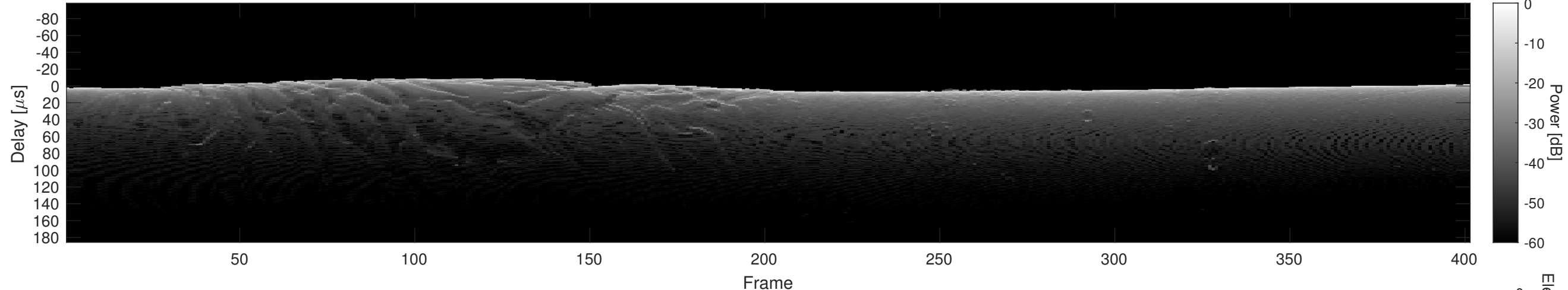
Orbit 18309, Cluttergram
