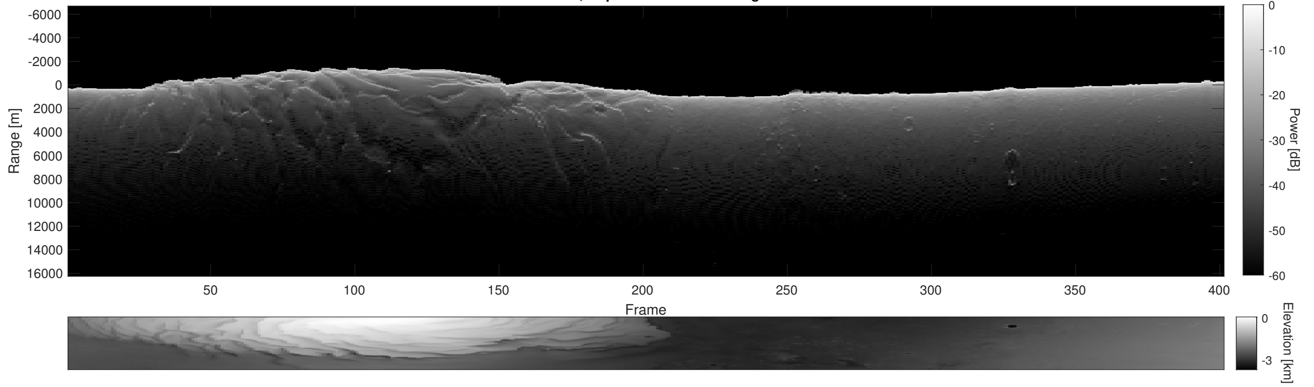
Orbit 18309, Depth-Corrected Cluttergram
