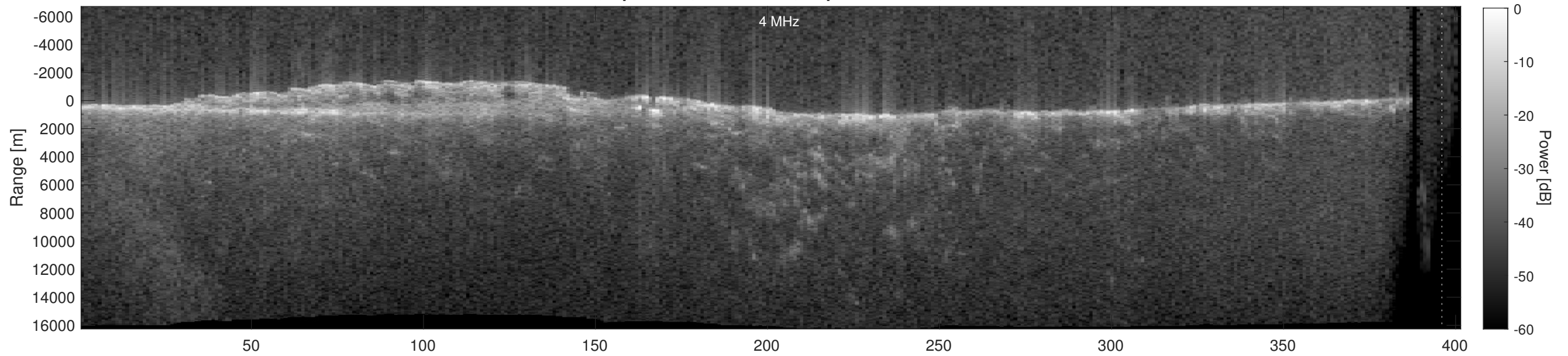
Orbit 18309, Depth-Corrected Cluttergram
