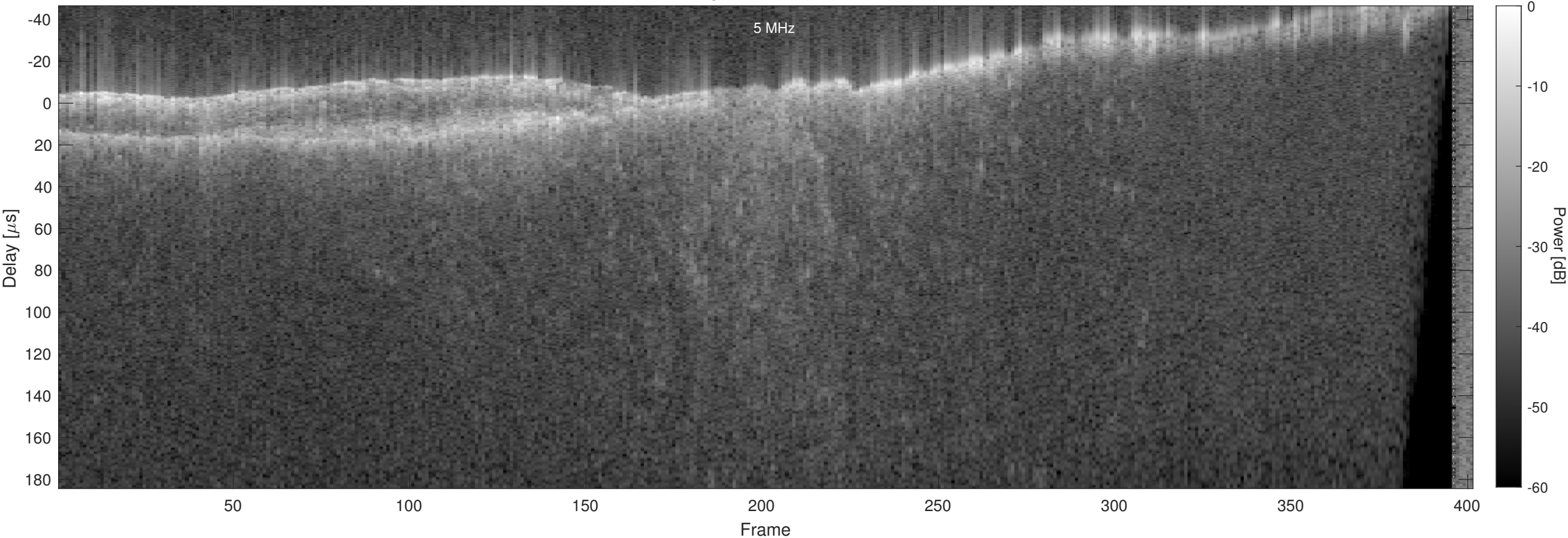
Orbit 18310, Chapman, No Window, Channel 2
