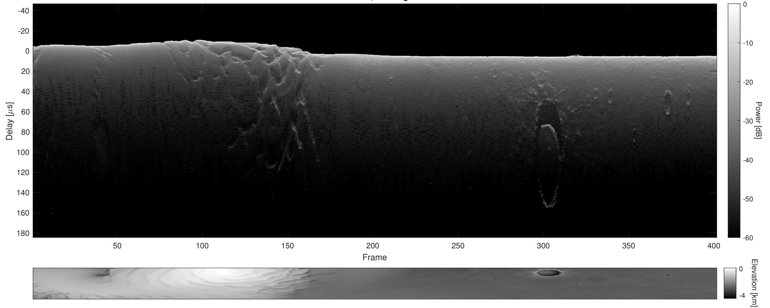
Orbit 18310, Cluttergram
