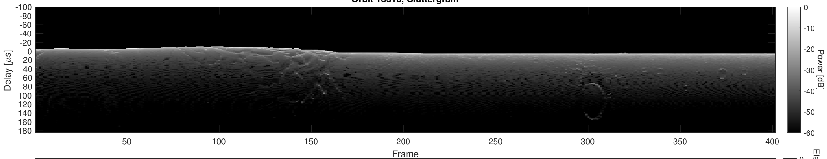
Orbit 18310, Cluttergram
