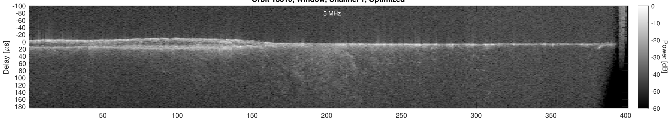
Orbit 18310, Cluttergram
