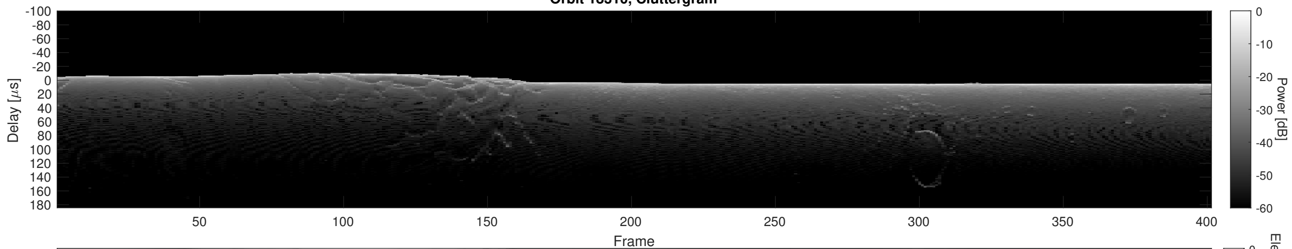
Orbit 18310, Cluttergram
