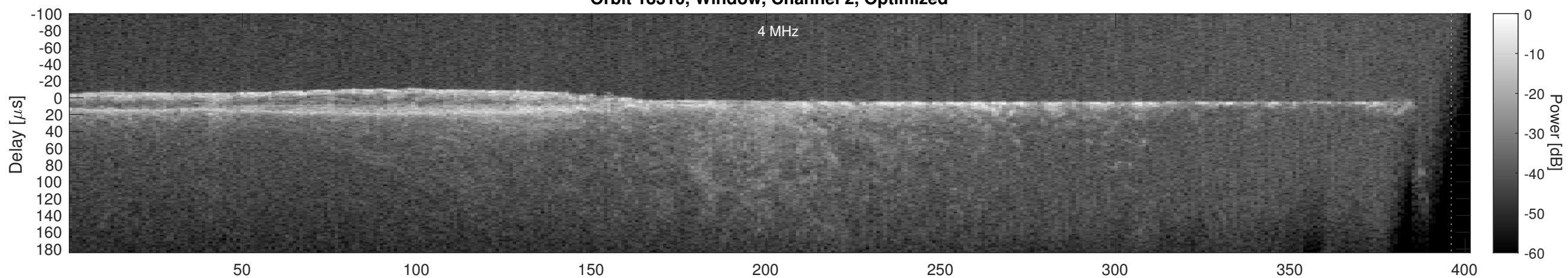
Orbit 18310, Cluttergram
